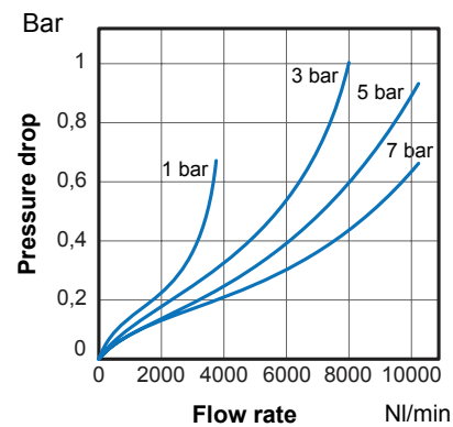
FLOW CHART FPLM04
