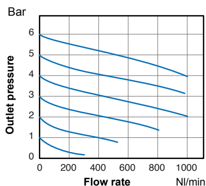
FLOW CHART FPFRPLP02 / FPFRLGPL02
