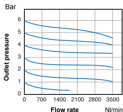
FLOW CHART FPFRMLM04 / FPFRLGLM04
