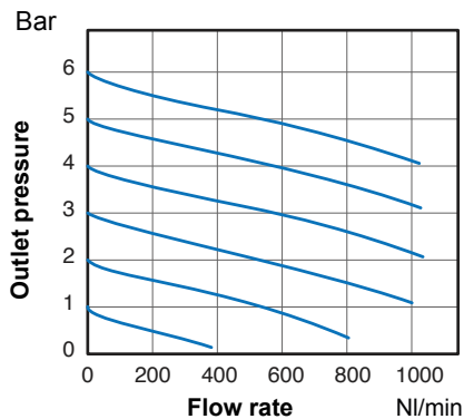
FLOW CHART FPFRP02 / FPFRPG02
