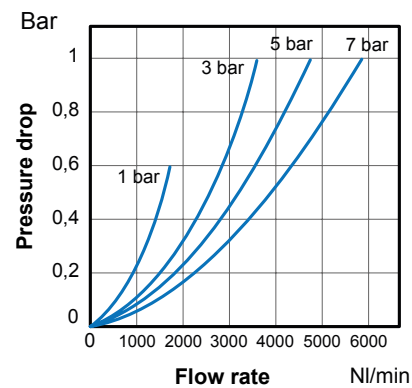
FLOW CHART FPFM04
